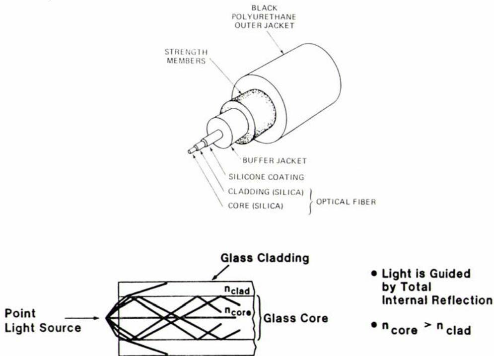
Figure 2.1: Schematic of an optical fiber.
