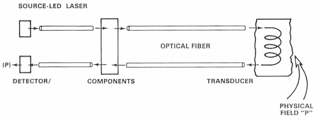
Figure 2.2: Basic elements of an optical fiber sensing system
