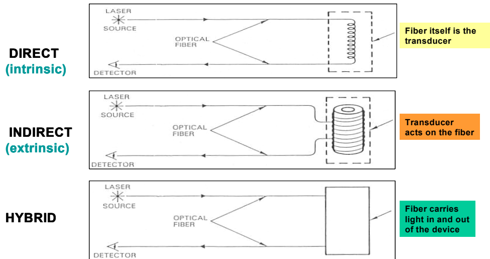
Figure 2.3: Classification of optical fiber sensors
