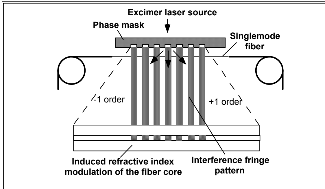
Figure 3.3 Phase mask technique for writing fiber Bragg gratings
