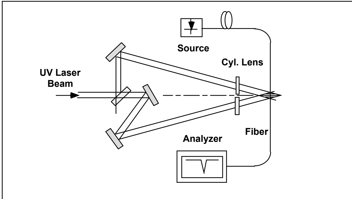
Figure 3.2 Two-beam interferometer for writing fiber Bragg gratings
