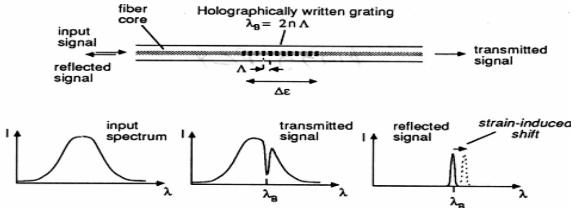
Figure 3.1. Transmission and reflection spectra of a fiber Bragg grating
