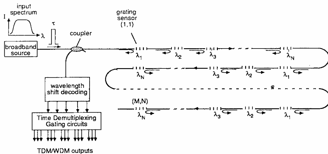
Figure 3.5 Aspect of a time-multiplexed WDM interrogated FBG sensor array
